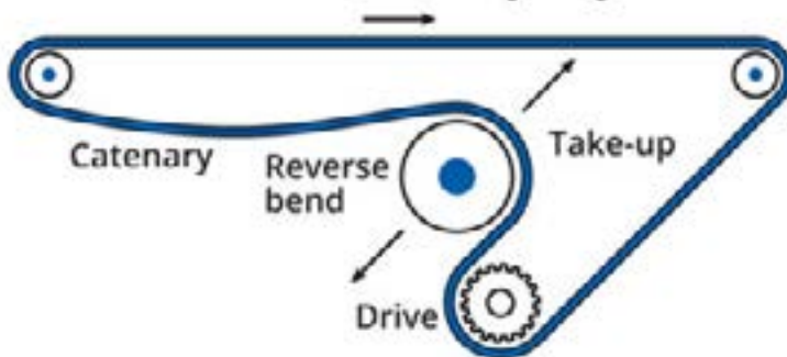
Alternate "S" Drive conveyor layout
